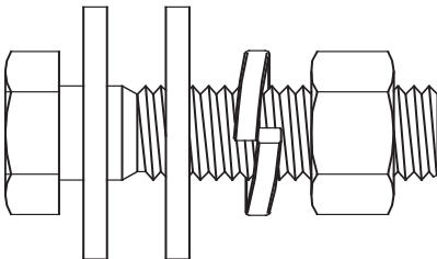
Rim Bolt Assembly (#7 in Parts List)
